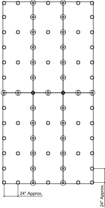
4' x 12' Grating Panels
