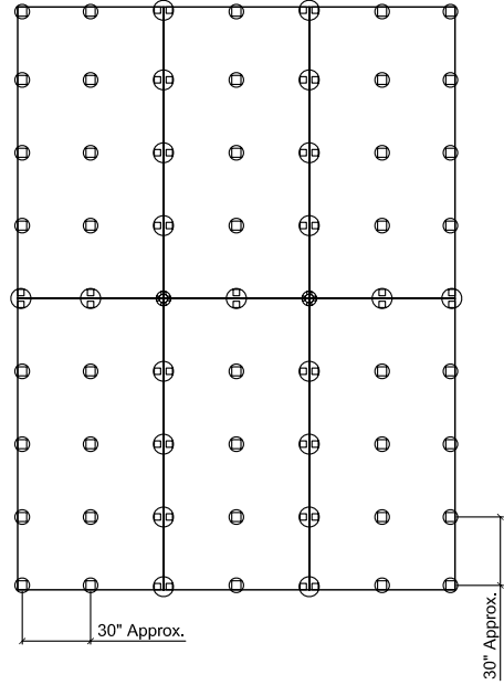
5' x 10' Grating Panels
