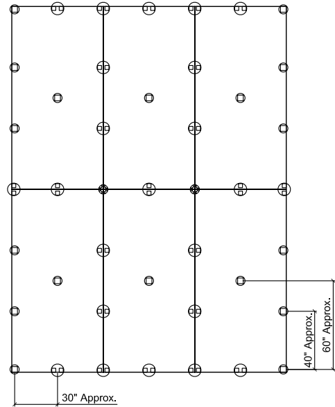
5' x 10' Grating Panels
